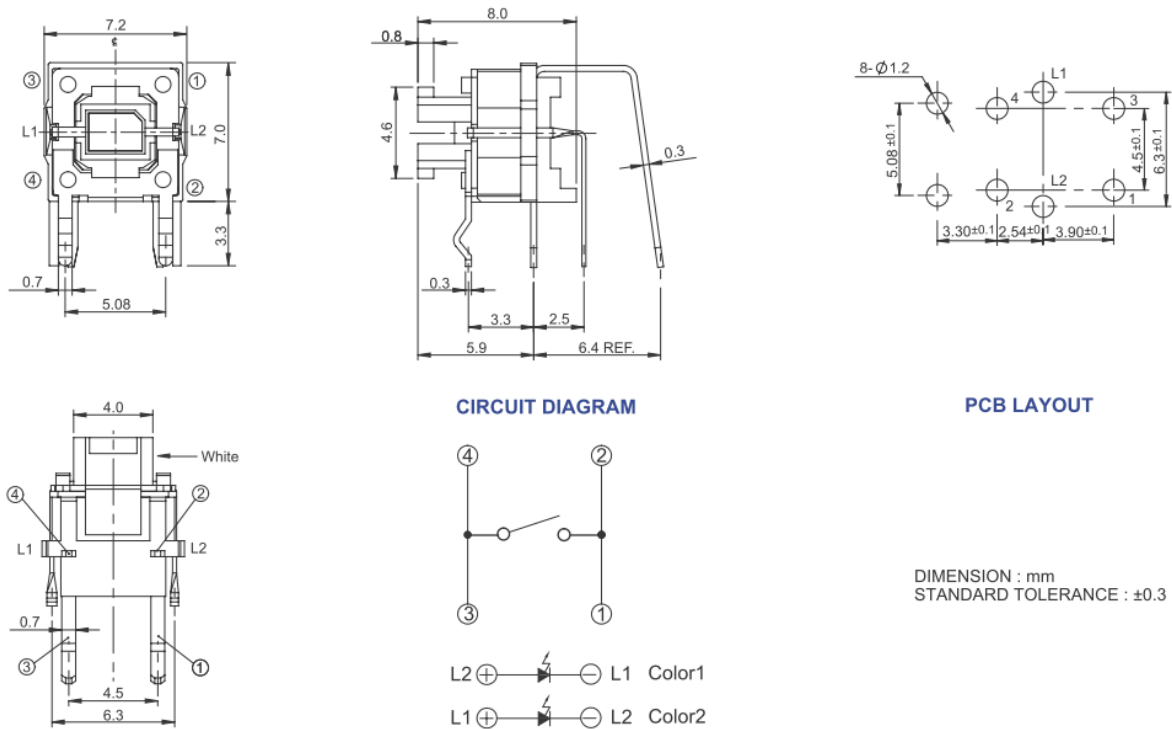
Figure 4 – 228ADVA...A..., Standard Though Hole, Vertical Actuation, Elliptical Column on Round Cap in Natural Color
